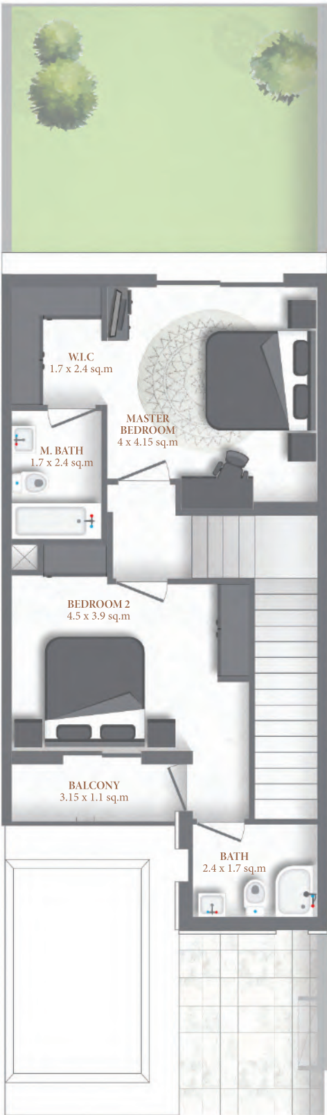
First Floor
